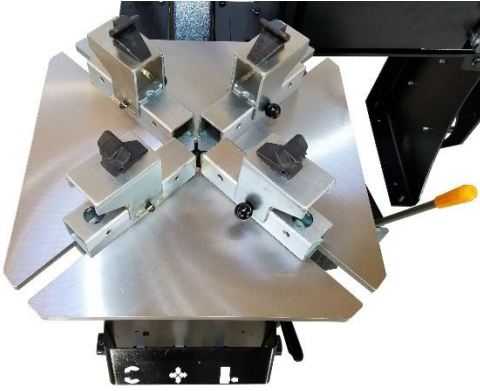
Unique Turntable Clamps Designed to Fit Motorcycle & ATV Rims with included Jaw Protectors
